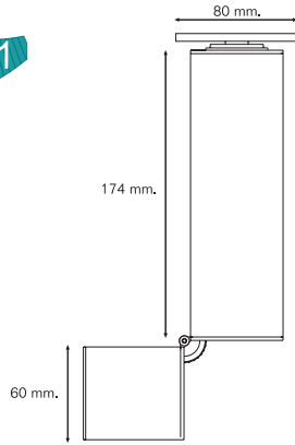
Deckeneinbauleuchte [recessed downlight] 503-150-..
